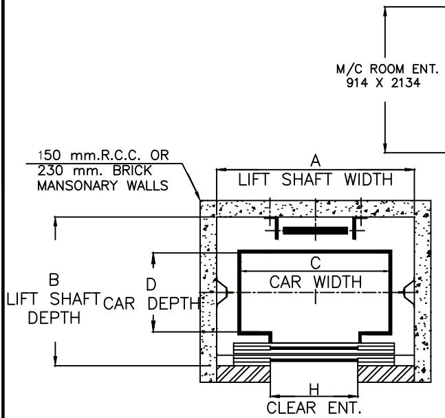
LIFT HOISTWAY PLAN
